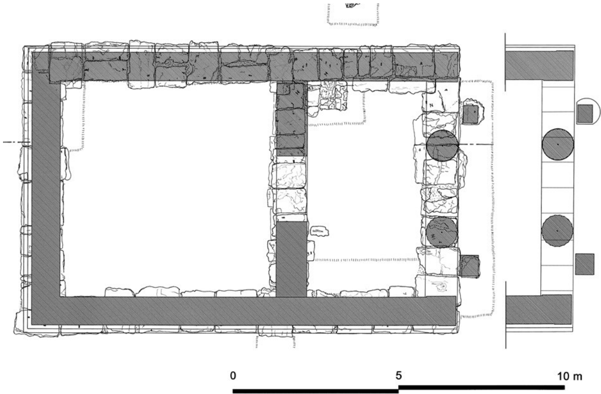
Fig. 28 Reconstructed plan of the Small Temple with in situ remains
