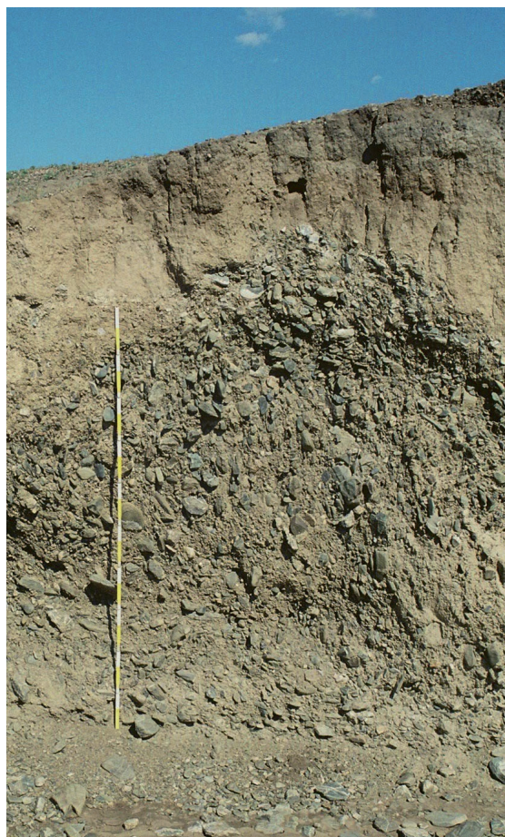
Fig. 4. Outcrop of the Orkhon terrace close to Kharkhorin exhibits fluvial deposits composed of basalt pebbles which are cryoturbatically reworked and covered by aeolian silts and sands.
