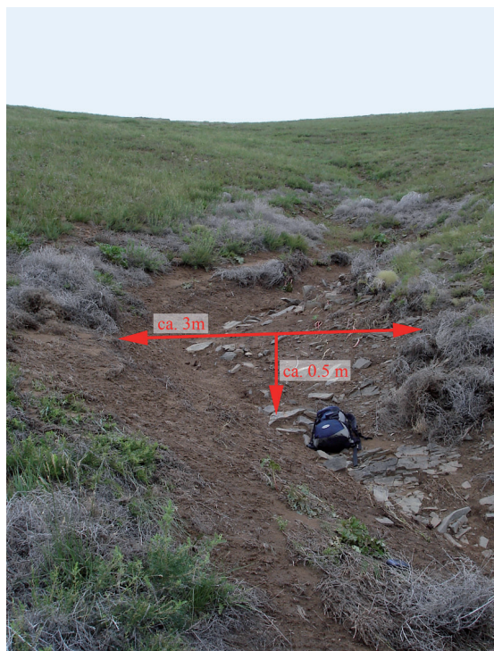
Fig. 8. Channel morphology at Ögii Nuur headwater area. The picture was taken one day after a heavy rainfall event. The site shown has a drainage area of around 0.5 km 2 .
